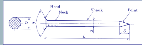
DIMENSION OF LOW CARBON STEEL WIRE NAIL
