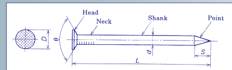
DIMENSION OF LOW CARBON STEEL WIRE NAIL
